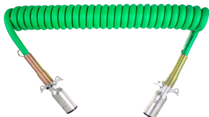
1/8, 2/10, 4/12 GA 7 CONDUCTOR ABS COILED 15FT WORKING LENGTH URETHANE ASSEMBLY NO ZINC PLUGS PART NO: TRA4AA15 PRICE: $84.50ea | QTY: 1
