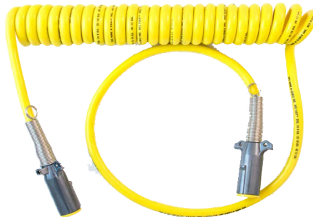
1/8, 2/10, 4/12 GA ISO MODIFIED YELLOW COILED CABLE 12FT WORKING LENGTH PART NO: TRA38604-12A PRICE: $35.00ea | QTY: 1
