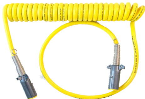
1/8, 2/10, 4/12 GA ISO MODIFIED YELLOW COILED CABLE 12FT WORKING LENGTH PART NO: TRA38604-12A PRICE: $35.00ea | QTY: 1
